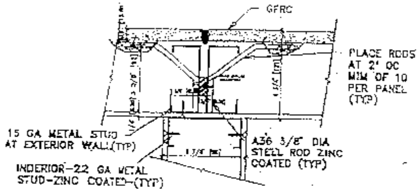
3 INTERIOR TO EXTERIOR WALL
