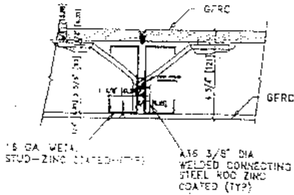
4 PANEL CONNECTION @ EXT. WALL
