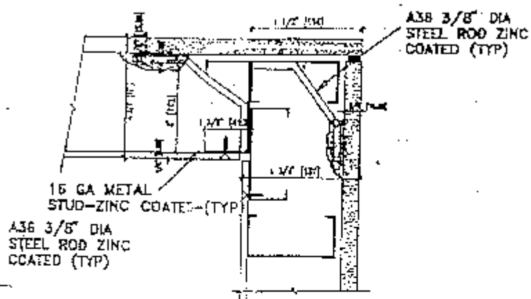
5 OUTSIDE CORNER @ EXT. WALL
